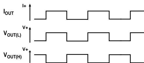
Figure 4: Voltages profiles for high side and low side two-wire sensing.
