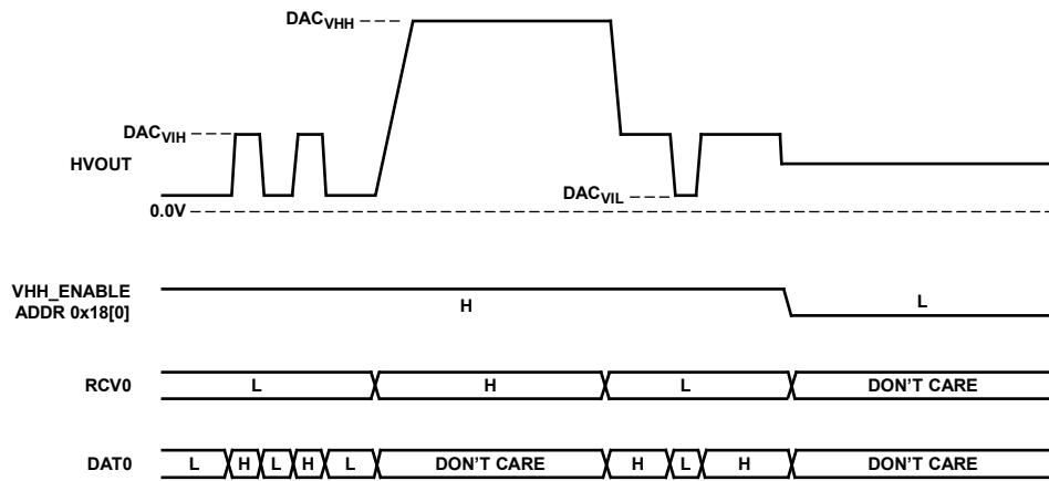
Figure 133. VHH and VIL/VIH Waveform Diagram
