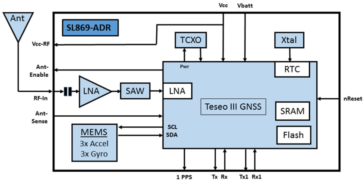
Figure 2-1 SL869-ADR Block Diagram
