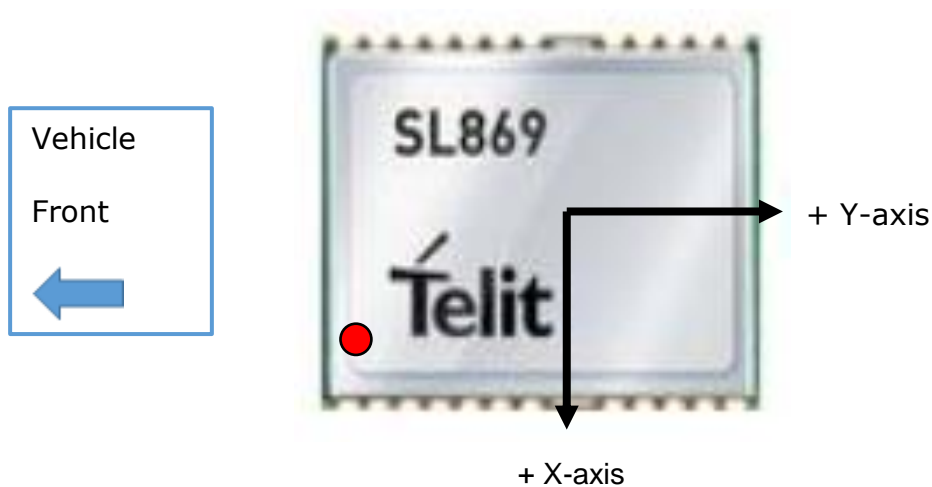
Figure 6-1 Module Orientation
