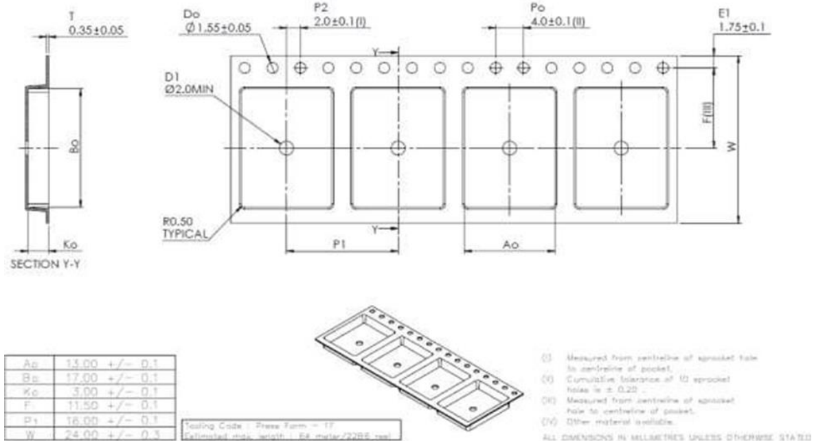
Figure 15-2 Tape and Reel Packaging
