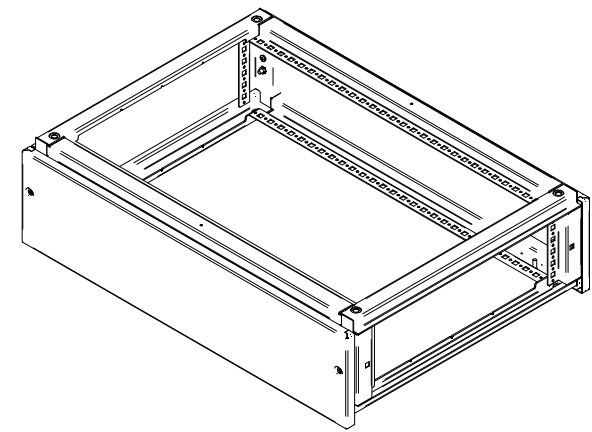
ISOMETRIC VIEW
