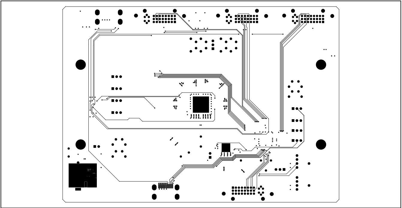
Figure 7. MAX3845/MAX4814E EV Kit Layout—Solder Plane
