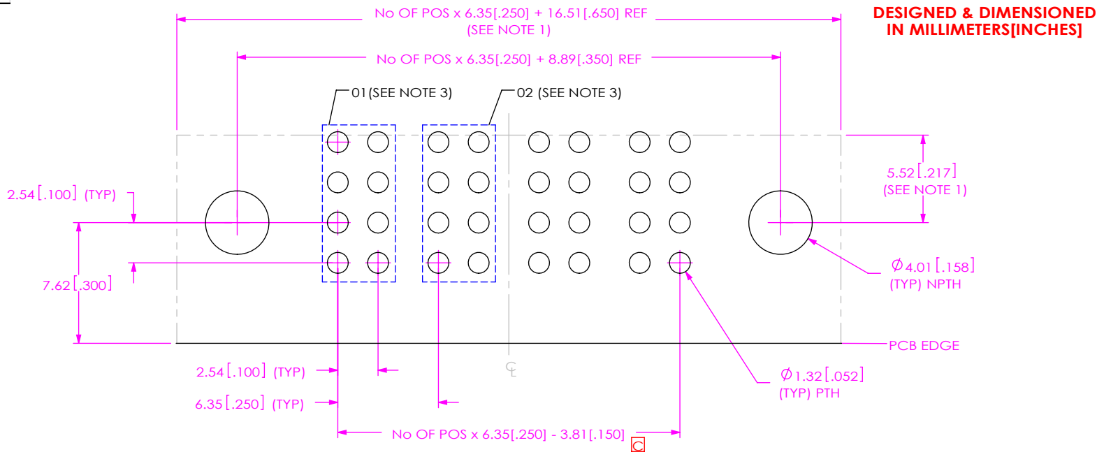
FIG 1 PCB LAYOUT FOR PET-XX-XX-XX-RA-SD SHOWN
