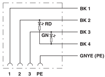
Contact assignment of the valve plug
